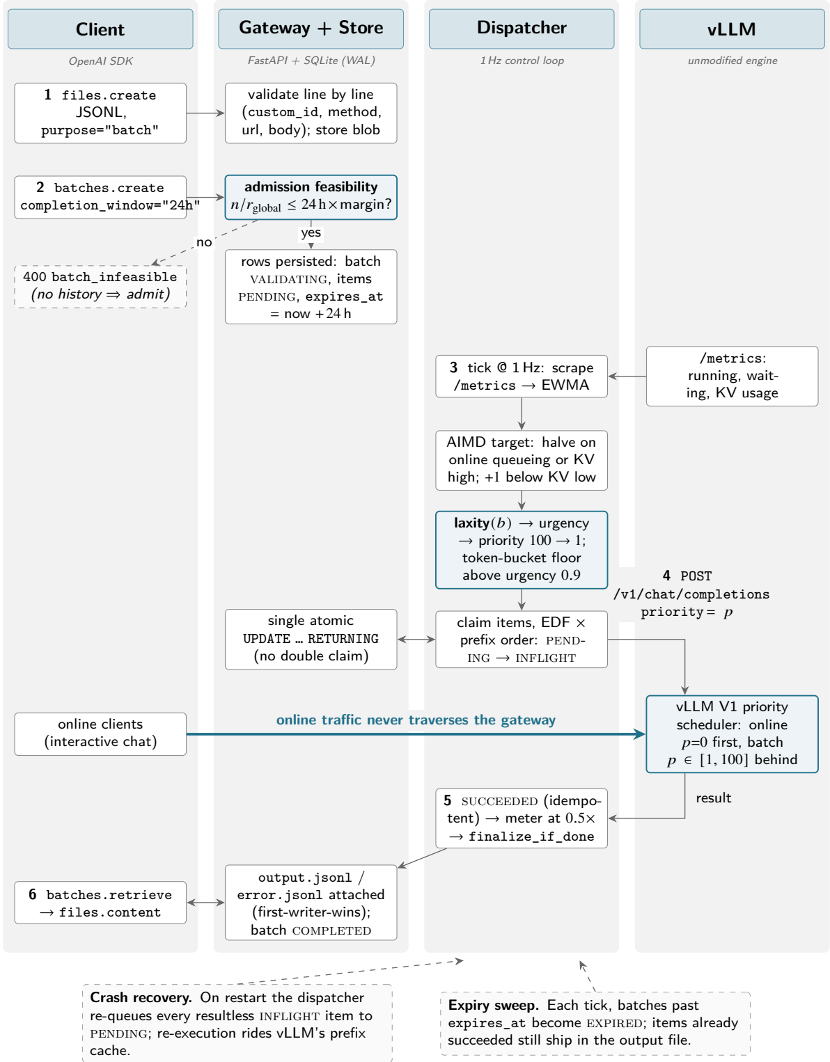
Figure 11: Technique A: the batch request lifecycle, end to end. A client uploads a JSONL file and creates a batch; the gateway validates every line and applies the laxity admission test, refusing with batch_infeasible any job whose projected completion exceeds the window times a margin, and otherwise persisting PENDING items with a 24-hour expires_at . A 1 Hz dispatcher scrapes the engine’s public metrics, sets an AIMD in-flight target, computes each batch’s laxity-derived priority, claims items in deadline × prefix order and submits them to vLLM as ordinary low-priority chat completions — while online clients (thick arrow) reach the engine directly, never through the gateway. Results settle idempotently, are metered at the batch discount, and are assembled into the output and error files the client downloads.
