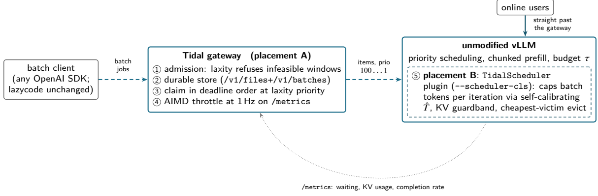
Figure 3: One policy, two placements. Batch jobs enter through an OpenAI-wire gateway that ① refuses infeasible windows at admission, ② stores jobs durably, ③ claims items in deadline order at their laxity priority, and ④ throttles dispatch by AIMD over the engine’s public metrics. Placement A stops there: the engine is stock vLLM, and online traffic never traverses the gateway. Placement B moves admission inside the engine ⑤ as a scheduler plugin that caps batch tokens per iteration against a self-calibrated latency model. Both are plugins; neither forks the engine.
