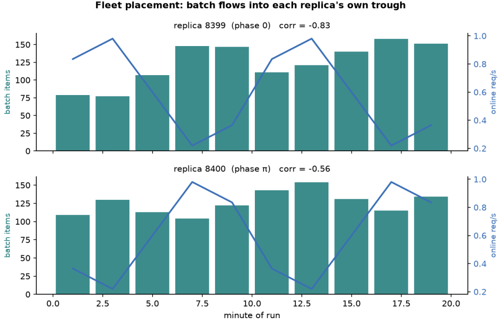
Figure 14: A-F mechanism, per replica: measured batch completions (bars) against each replica’s own analytic online rate (line). Volume splits evenly; timing follows each replica’s trough.
