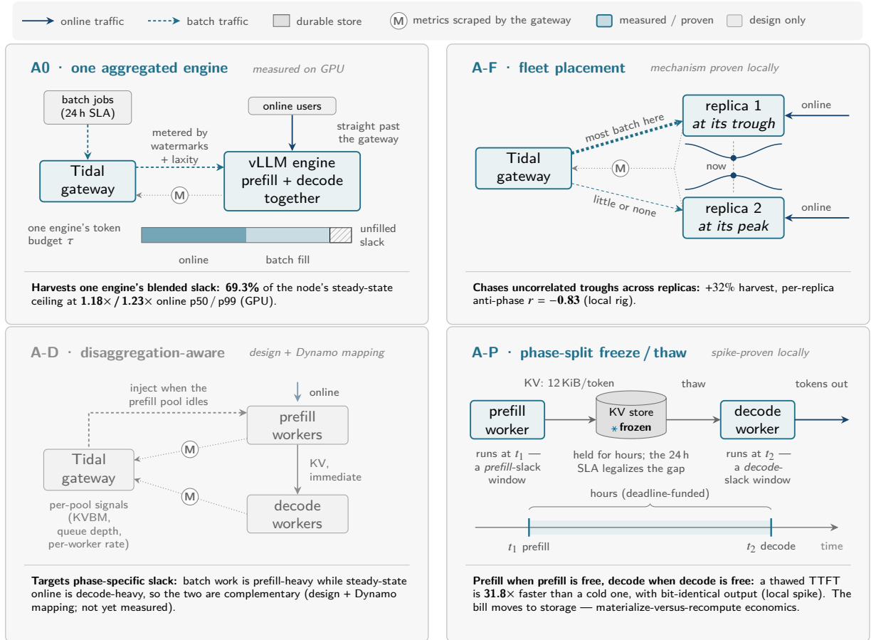
Figure 13: The A-ladder, drawn. The four rungs of Table 6, in order of widening scope: A0 places deferrable work inside one aggregated engine, A-F across the replicas of a fleet, A-D into the idle phase pool of a disaggregated deployment, and A-P across time itself, by freezing a finished prefill’s KV to a durable store and thawing it into a decode worker hours later. Each panel carries the advantage that rung buys and the number that evidences it; A-D is drawn dimmed because it is design plus a metric mapping (Table 8) rather than a measurement. The last rung makes the section’s one-liner literal: disaggregation separates prefill from decode in space; a deadline-contracted batch tier separates them in time.
