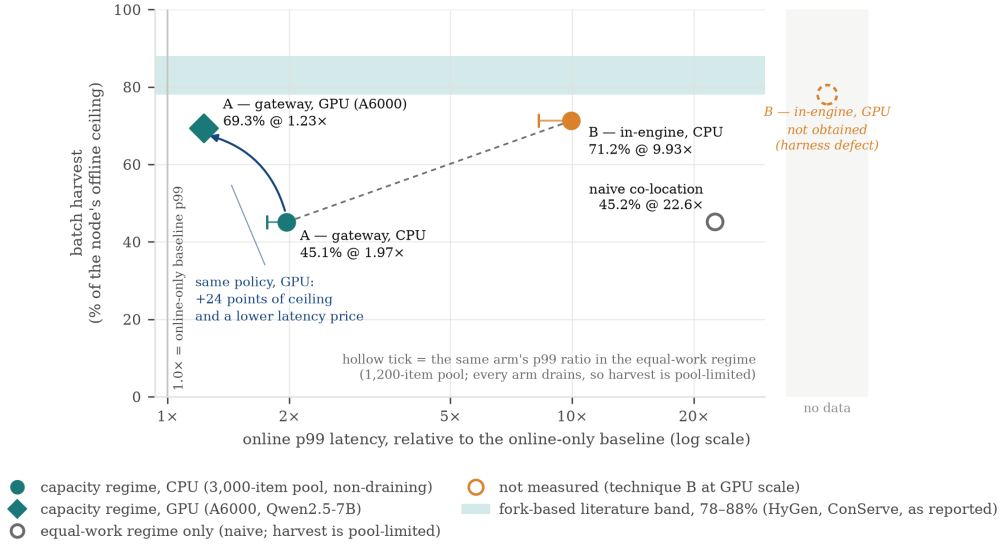
Figure 9: Placement is a frontier, not a ranking. Online p99 ratio (log) against harvest, all measured arms, with the band the fork-based literature reports shaded. The same policy moves from the CPU point to the GPU point when the binding resource changes; technique B’s GPU point was not obtained (open marker).
