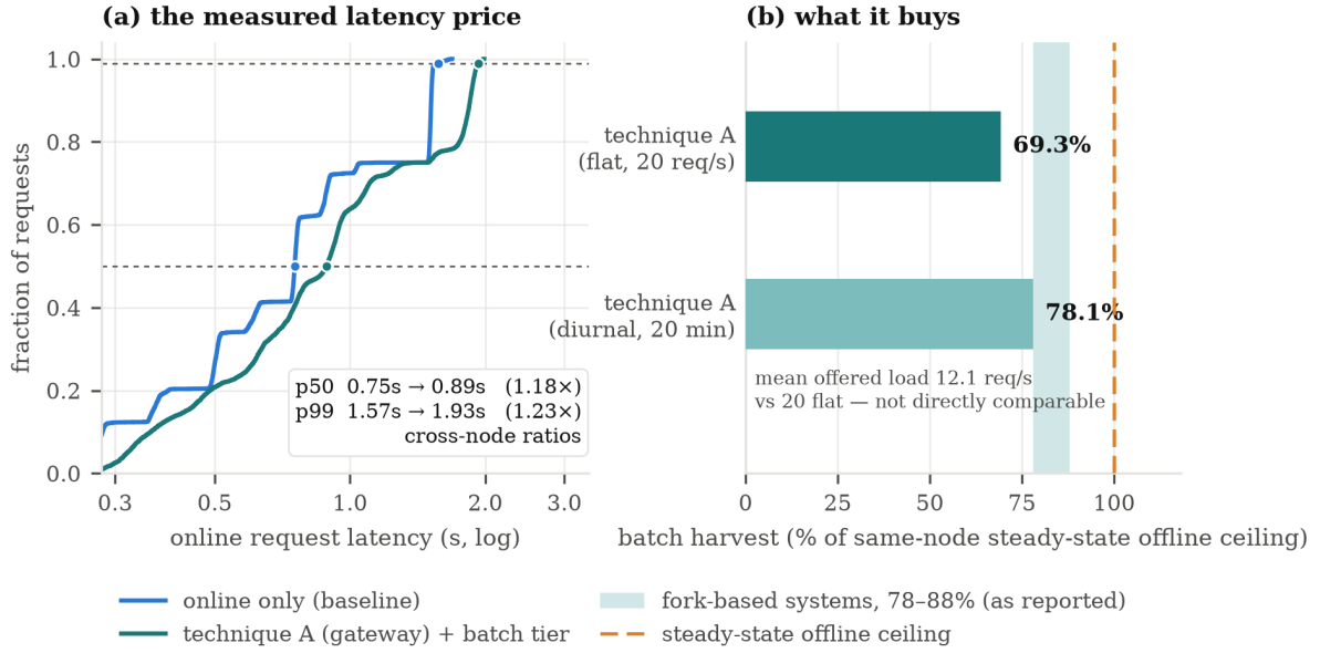
Figure 6: The headline trade at GPU scale. Left: online request-latency CDF, baseline versus technique A (cross-node). Right: batch harvest as a fraction of the node’s steady-state offline ceiling, with the band the fork-based literature reports shaded for reference.
