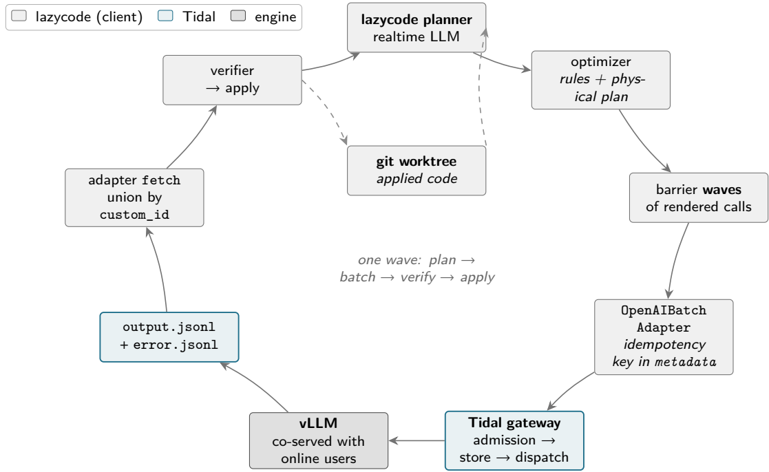
Figure 12: The complete loop. A realtime model plans the work; the optimizer lowers the plan into barrier waves of rendered calls; the OpenAIBatchAdapter uploads a wave as JSONL and stamps a server-side idempotency key in the batch’s metadata, so a crashed run can adopt its own orphaned batch. Tidal admits, stores and dispatches the wave into a vLLM that is simultaneously serving online users; the adapter fetches the output and error files and reassembles the wave by union over custom_id; the verifier runs the results and applies what passes into a git worktree, which feeds the next wave. This is the request lifecycle from client intent to applied code, entirely on self-hosted capacity at batch pricing. The client-side stages (planner, optimizer, waves, verifier) are detailed in the companion paper [29]; this figure shows only their interface to the serving tier.
